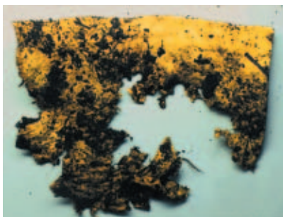
After 5 weeks: Sample shrunken, about 60% dissolved
